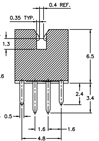
SECTION A-A SCALE 5:1
