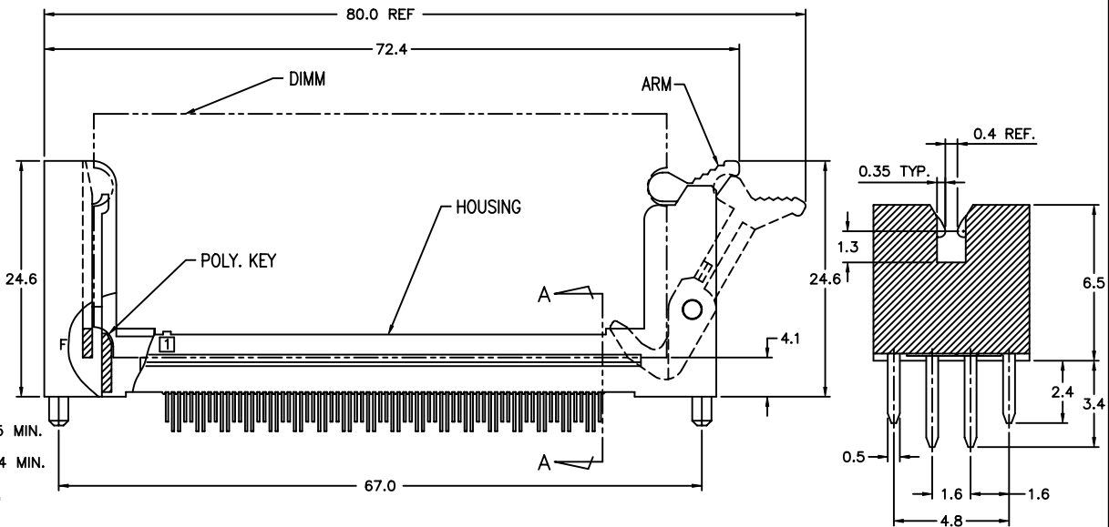
SECT. A-A SCALE 5:1
